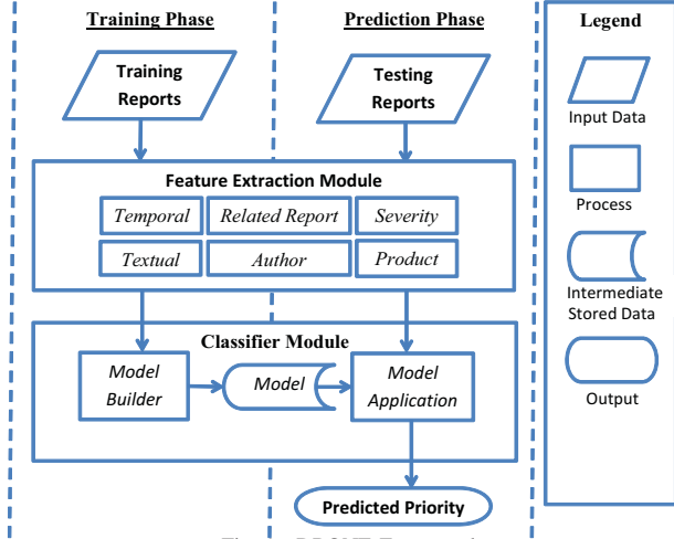
Fig. 1. DRONE Framework
